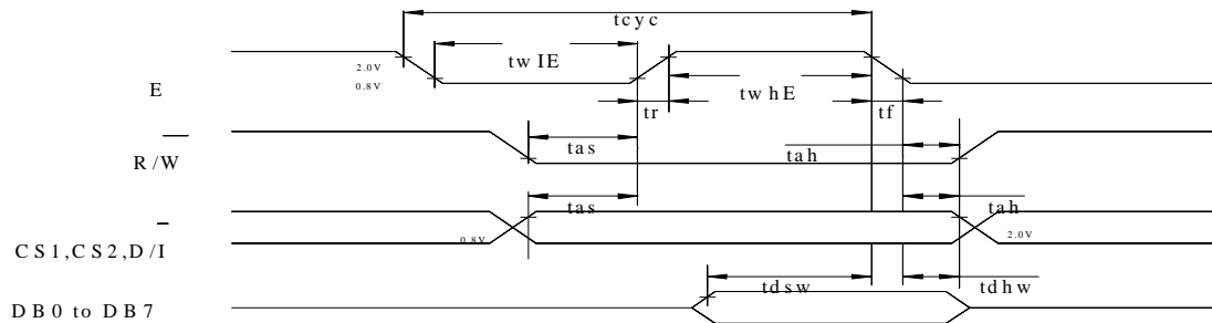
MPU Write Timing
